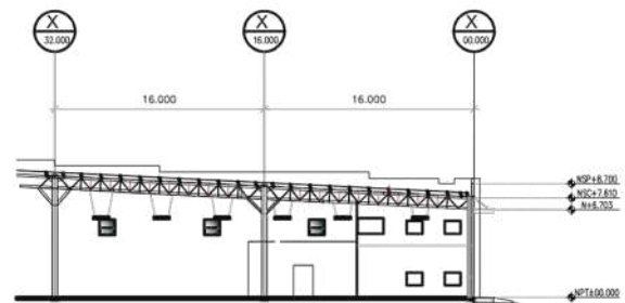
BUILDING SECTION
